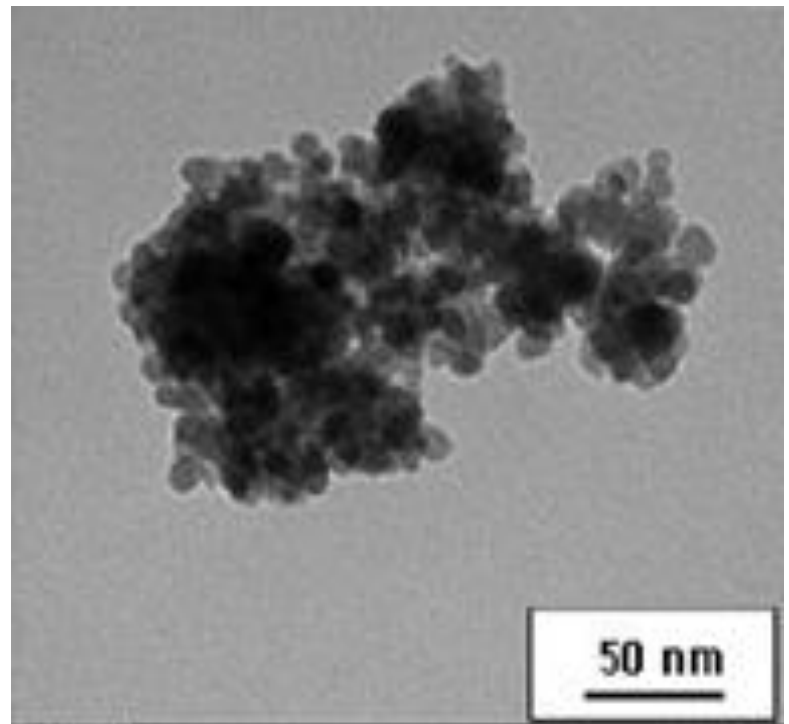
amino-MNPs powder
