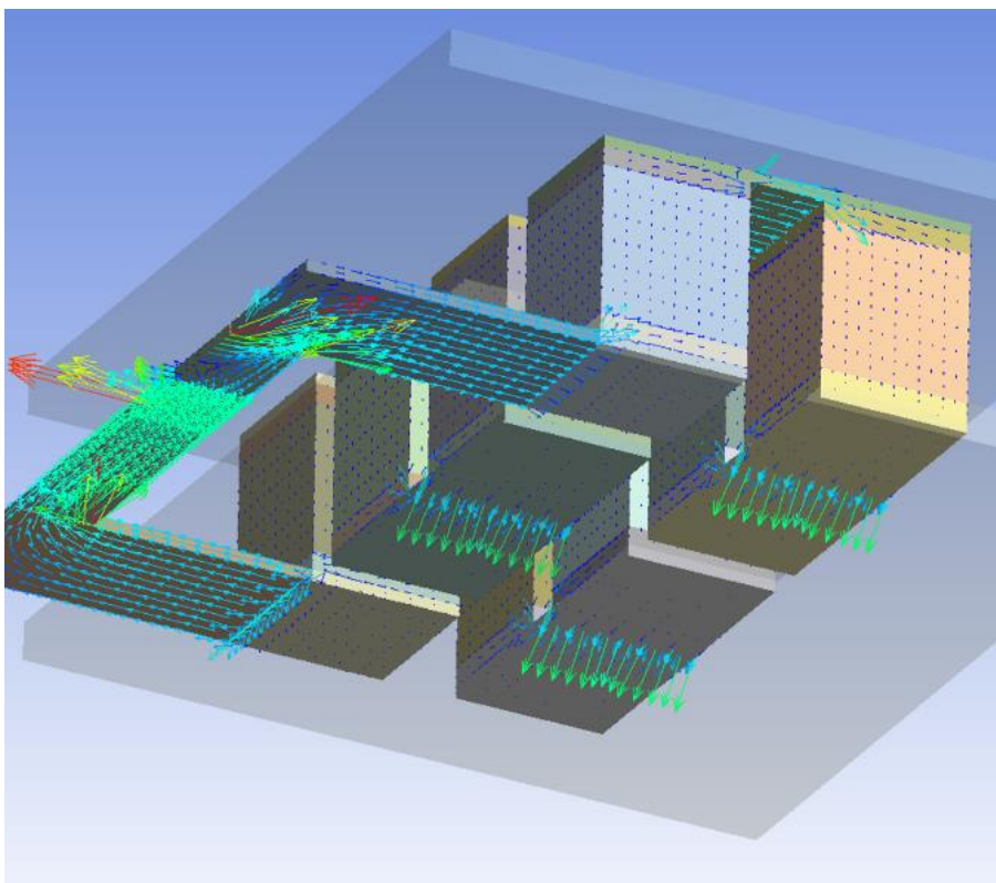
Thermoelectric module simulation by Finite Element Method
