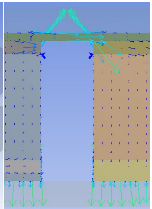
Thermoelectric module simulation by Finite Element Method
